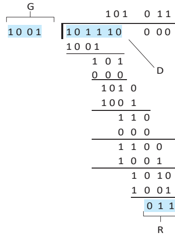
Figure 5.7 ♦ A sample CRC calculation
