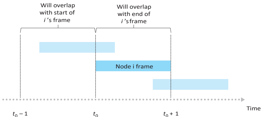
Figure 5.11 ♦ Interfering transmissions in pure ALOHA
