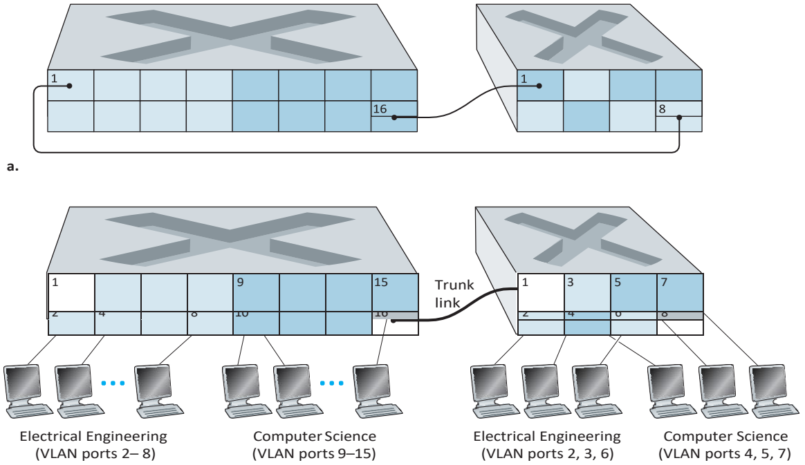
b. Figure 5.26 ♦ Connecting two VLAN switches with two VLANs: (a) two cables (b) trunked
