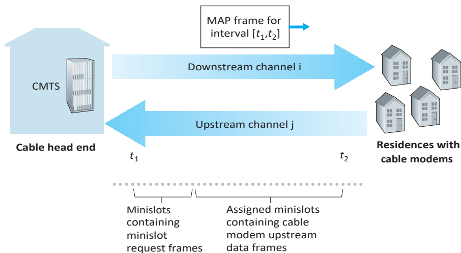
Figure 5.14 ♦ Upstream and downstream channels between CMTS and cable modems
