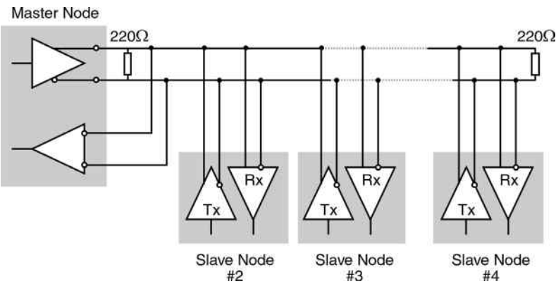
Figure 1.4 RS-485 Connection
