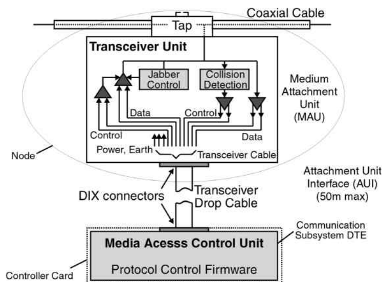
Figure 2.6 10BASE-5 Hardware Components
