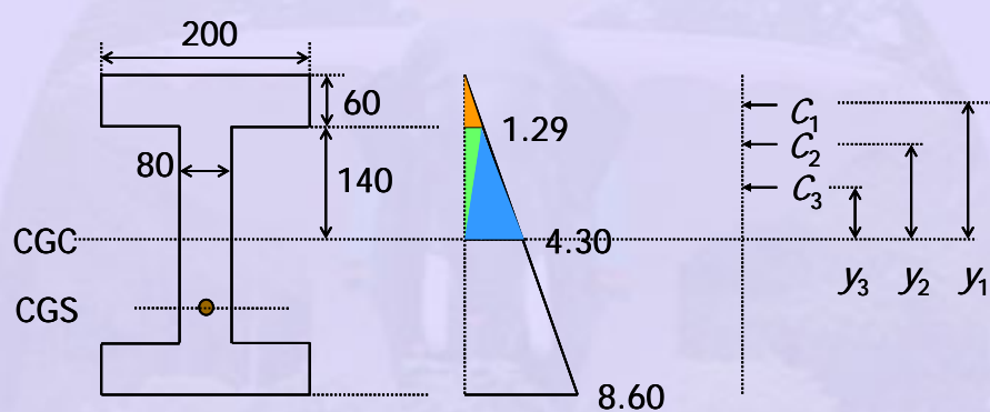
Stress profile
