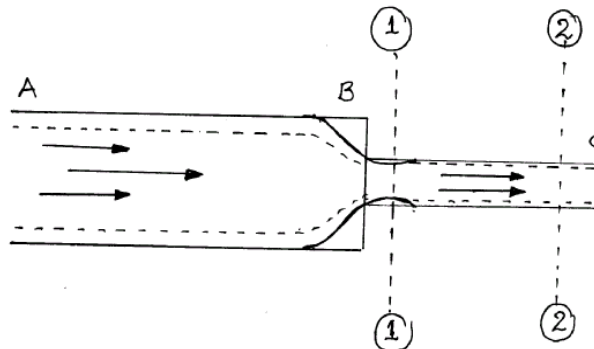
Fig 10.2 Sudden Contraction
