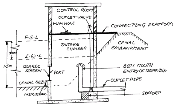
Fig. 3.14 Canal Intake
