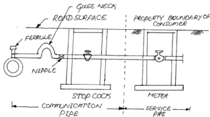
Fig 8.1 House water connection
