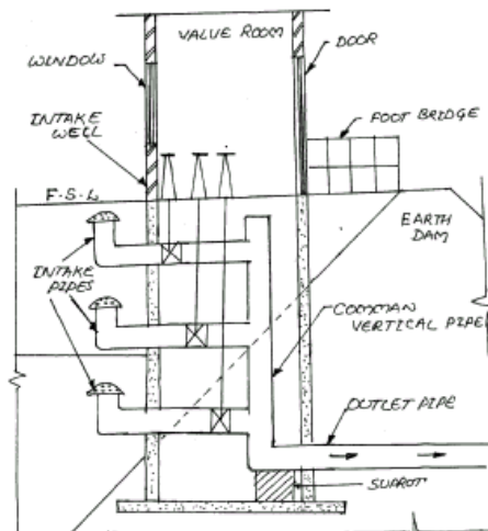
Fig. 3.13 Reservoir Intake
