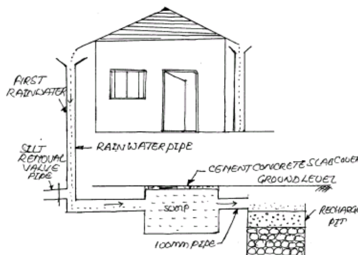
Fig 9.1 Storage Sump and Recharge Pit
