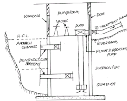
Fig. 3.12 River Intake
