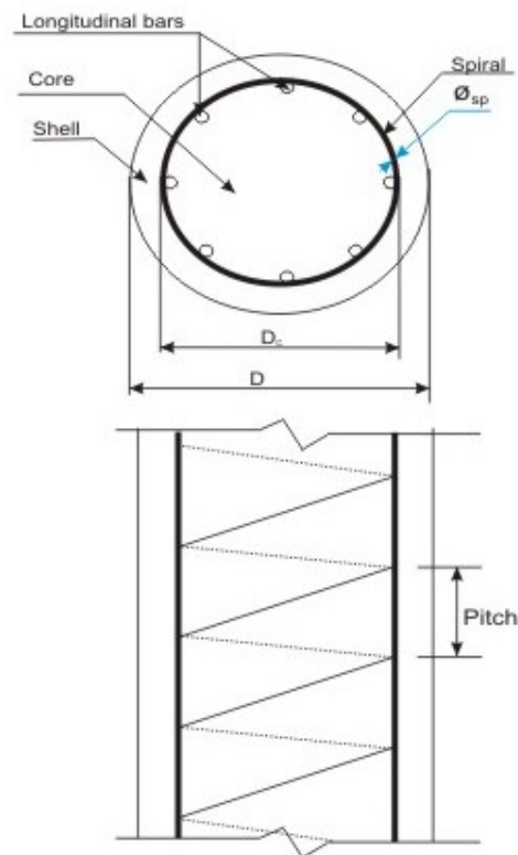
Fig. 10.21.2b: Column with helical reinforcement
