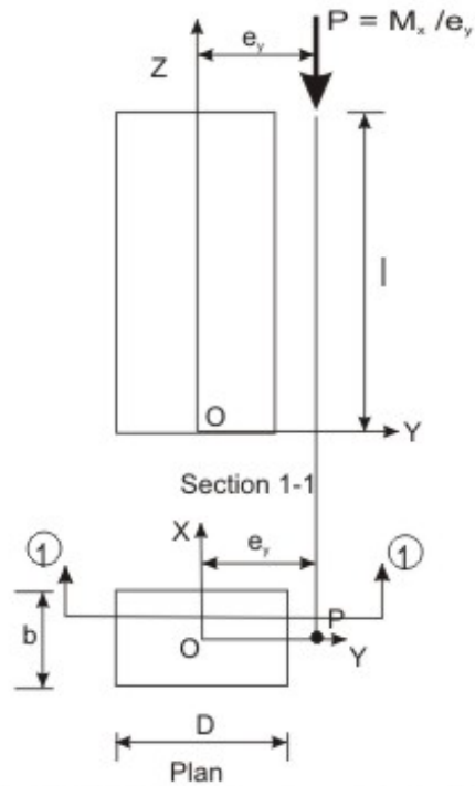
Fig. 10.21.3(b): Axial loading with uniaxial bending
