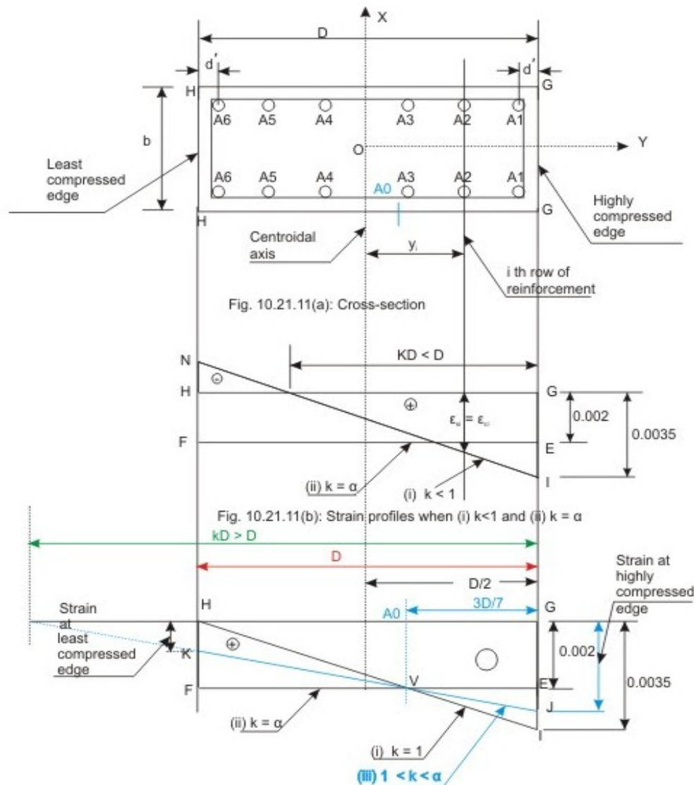
Fig. 10.21.11: Strain profiles for different positions of neutral axis
