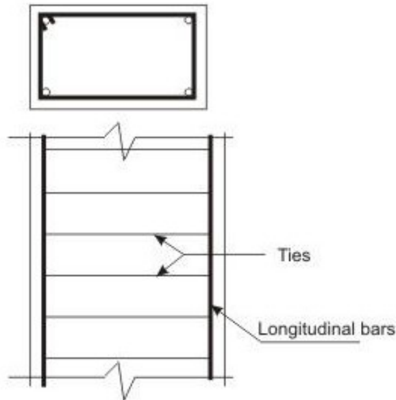
Fig. 10.21.2(a): Tied column
