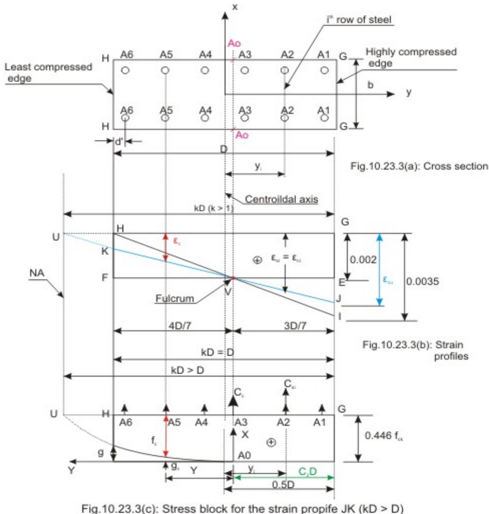
Fig.10.23.3: Cross section of column, strain profiles and stress block for the strain profile JK ( kD > D )
