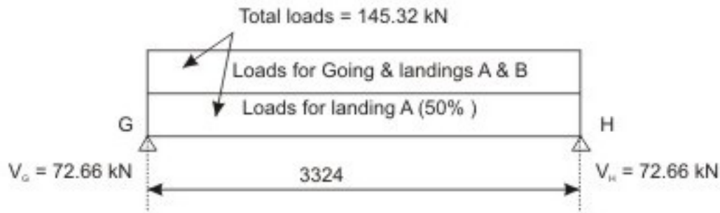
Fig. 9.20.19: Loads and reactions (Example 9.2 )
