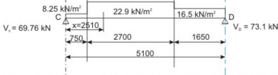
Fig. 9.20.11: Calculation of loads, sec 1-1 of Example 9.1, (Fig. 9.20.10)
