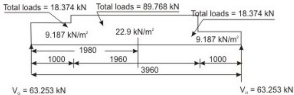
Fig 9.20.24: Calculation of loads, sec 2-2 of Fig. 9.20.21, Example Q.8
